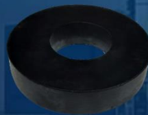
DONA REDUCTORA DR3X15 3 X 1.5" ETR3020 3" A 2" ETR4015 4" A 1.5" ETR4020 4" A 2" ETR6040 6" A 4"
